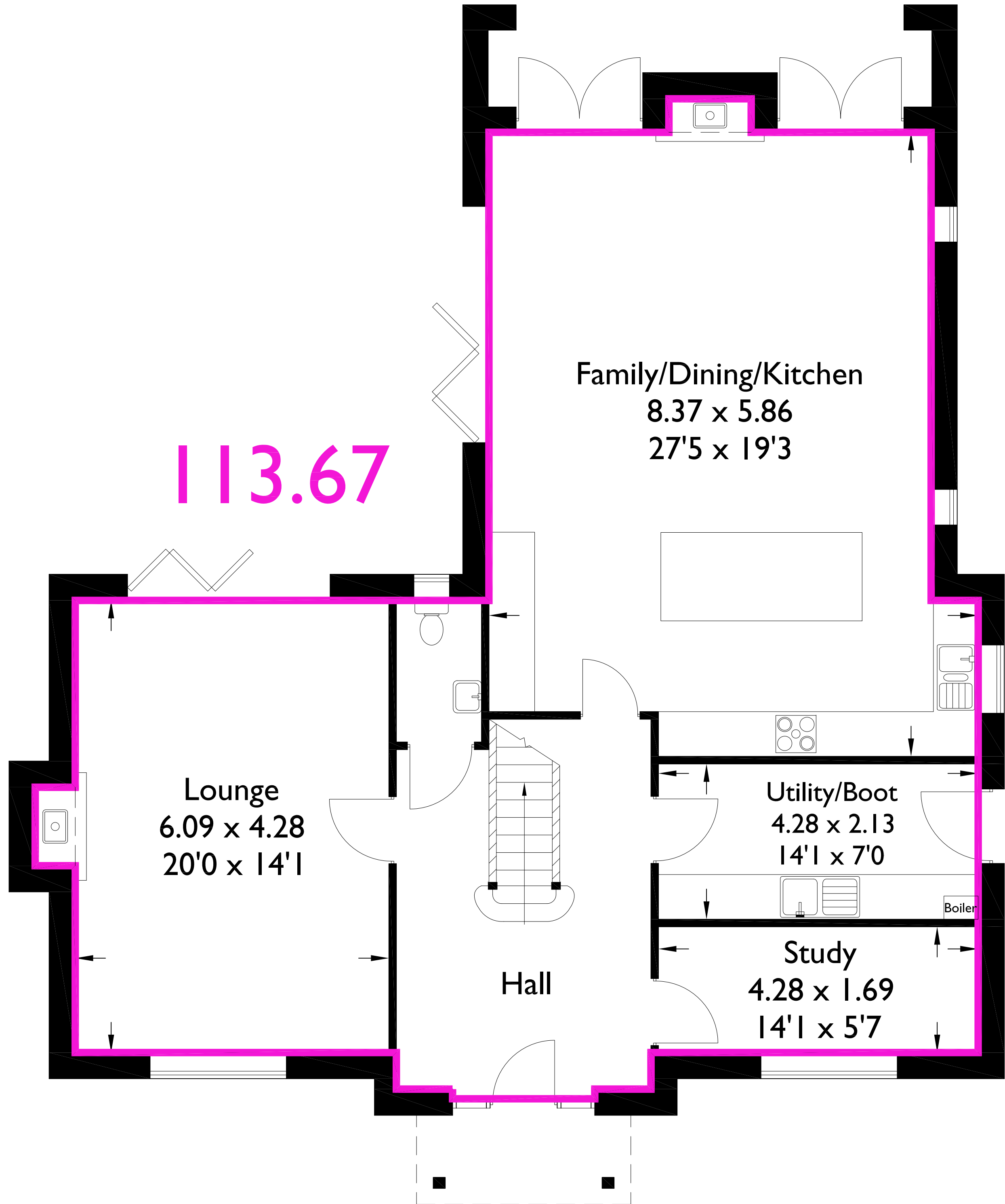
Ground Floor
