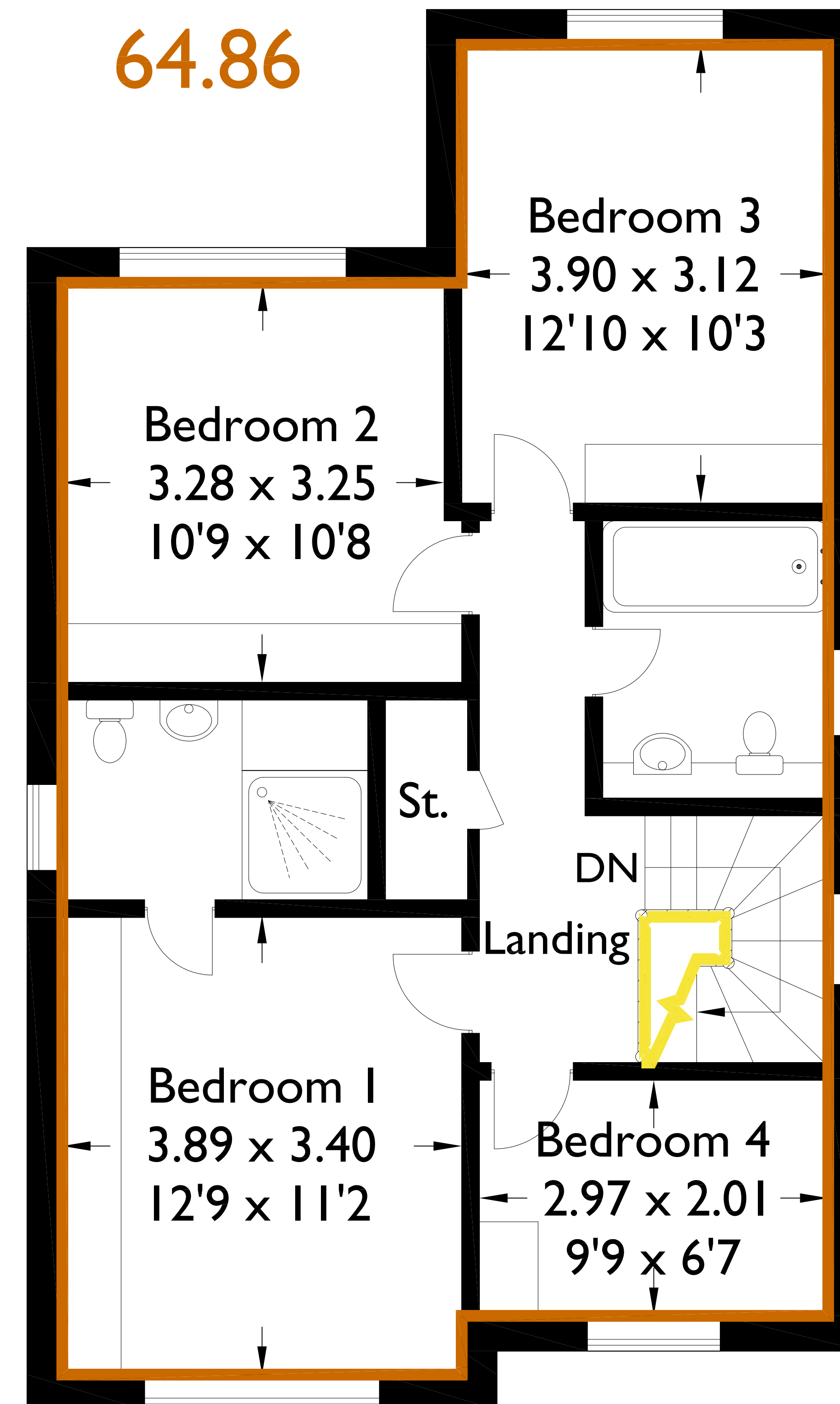
First Floor
