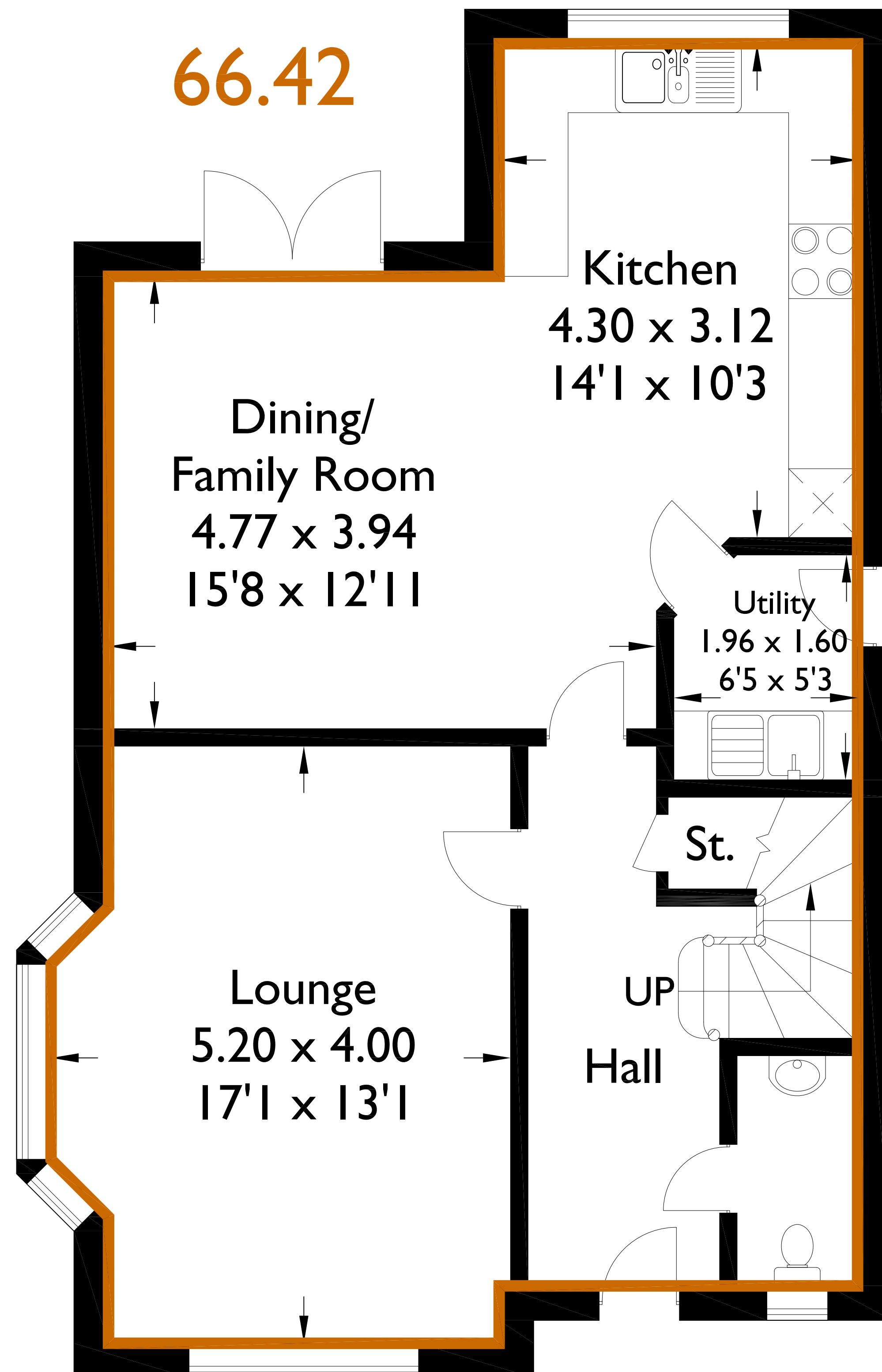
Ground Floor
